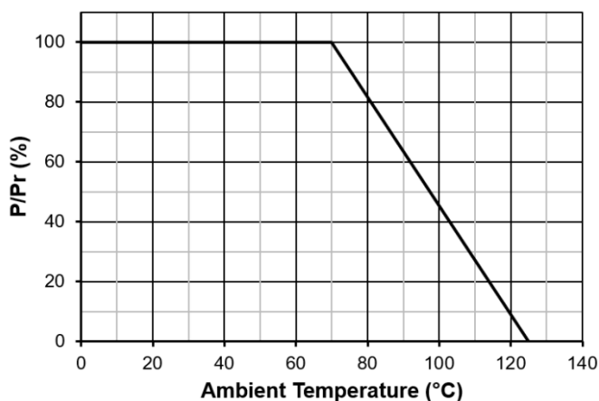
Temperature Derating
