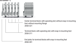
Example of a 5-pole terminal strip, with operating slot, with snap-in mounting feet Page number: 2
