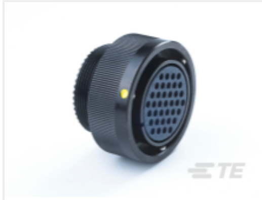
TE Part #Y5015-000000100034 FREE SOCKET CONNECTOR
