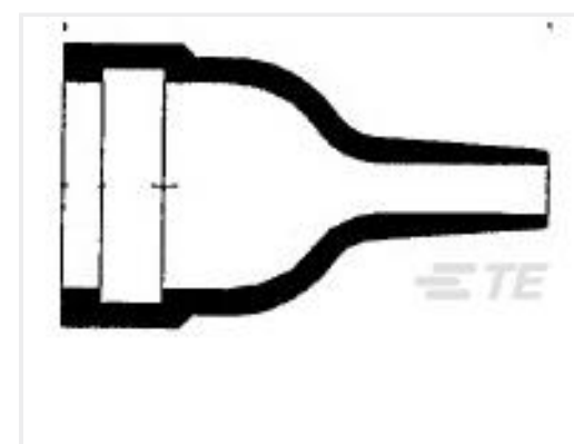
TE Part #D06723-000 204W221-12-0
