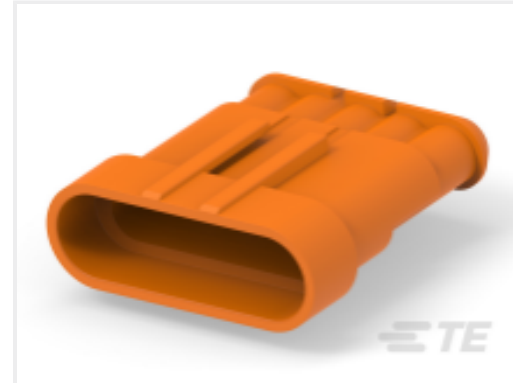
TE Part #1745018-1 SUPERSEAL 5 POS. TAB HOUSING (CLOSED CAV)
