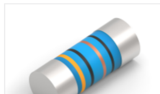
TE Part #3-2176314-0 MELF SMA_A 27K 0.1% 15PPM 0102 0.3W
