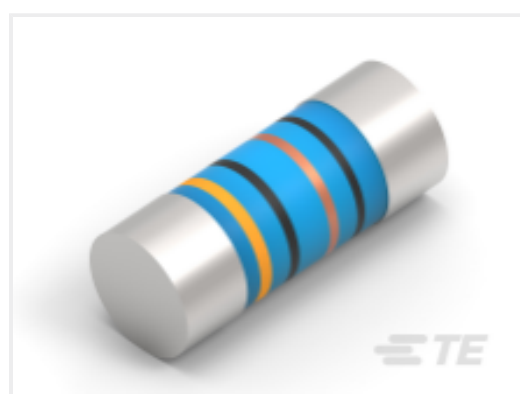
TE Part #5-2176316-8 MELF SMA_A 4K7 1% 50PPM 0207 1W
