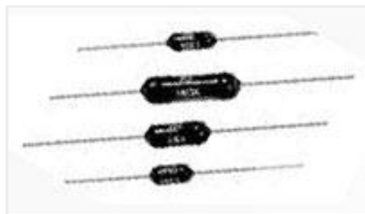
TE Part #8-1879663-6 H8 825R 0.1% 15PPM
