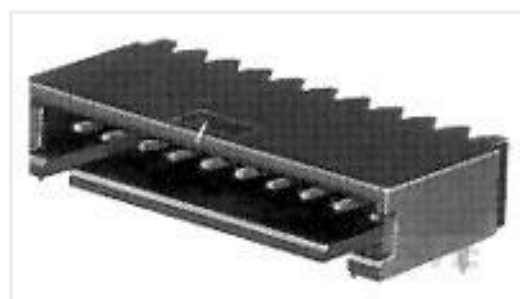
TE Part #5-103361-2 04 MODII HDR SRRR SHRD LF
