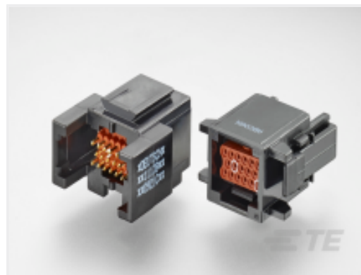
TE Part #ABC03N-20S-4048 IN-LINE RECP
