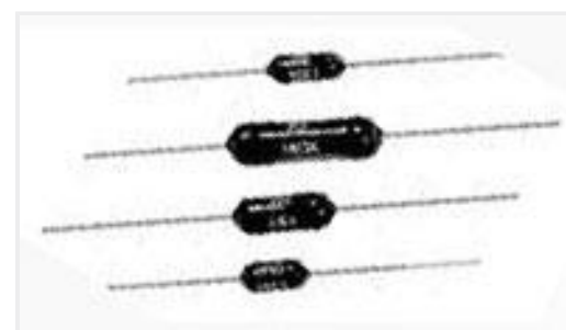
TE Part #7-1879625-1 H8 8K2 1% 50PPM
