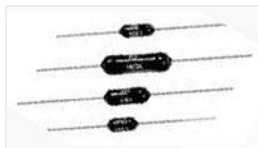
TE Part #4-1879645-7 H8 90R9 0.5% 50PPM
