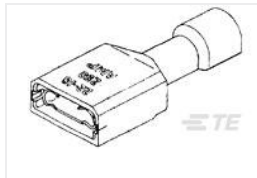
TE Part #2-520310-2 ULTRA-FAST .110/.125 ASY REC 22-18 TPBR
