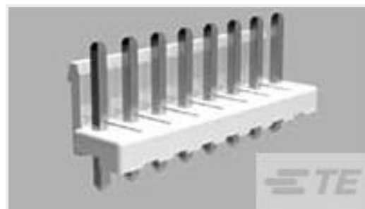
TE Part #4-1123723-4 3.96 EP HDR ASSY 4P(RED)
