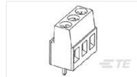
TE Part #282843-8 TERMI-BLOK PCB MOUNT 90 8P.1
