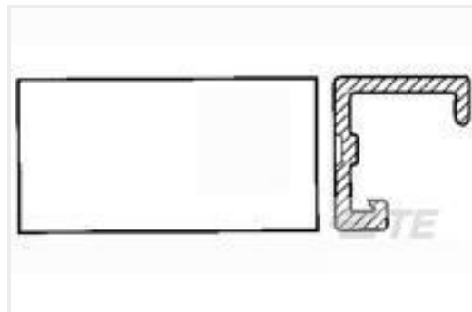
TE Part #1-640550-3 13P MTA100 COVER
