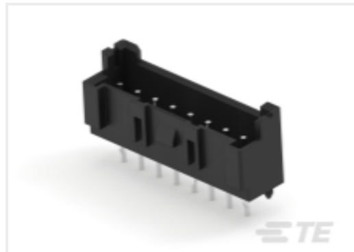
TE Part # 4-2338245-8 EP2.5 HDR 8P VERT BOSS, BLACK,UL
