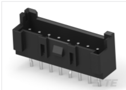
TE Part # 4-2338244-8 EP2.5 HDR 8P VERT W/O BOSS, BLACK,UL
