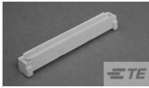
TE Part #2-5177986-6 0.8FH,P07H.5,140,08/Sn,TR,SC
