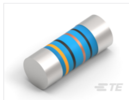
TE Part #3-2176316-8 MELF SMA_A 100R 1% 50PPM 0207 1W
