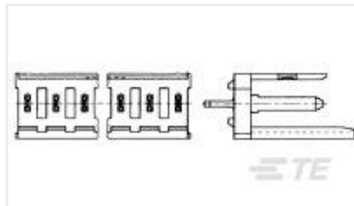
TE Part #280617-1 06P MOD 1 P.S.ASSY
