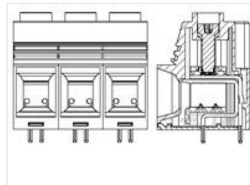
TE Part #1986242-4 Power Connector, 15.0mm, Green, 4 posn
