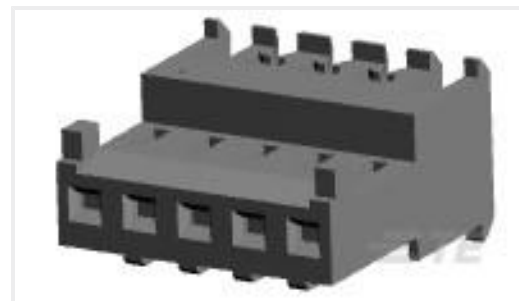
TE Part #3-644540-5 05P MTA100 CONN ASSY F/T W/LCK ORA
