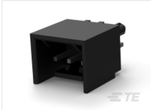
TE Part # 2-644487-3 03P MTA100 SHRD HDR ASSY 30AU
