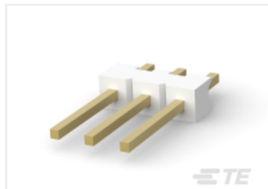
TE Part # CAT-104MTA-PVBRH Polyester Vertical PCB Header: 2.54 mm, Breakaway, MTA 100
