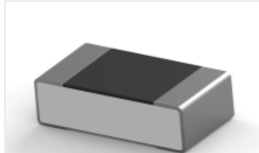
TE Part #2176370-7 RQ 0603 499R 0.1% 10PPM 5K RL
