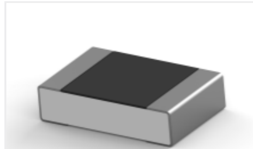
TE Part #2176380-5 RQ 0805 1K27 0.1% 10PPM 5K RL
