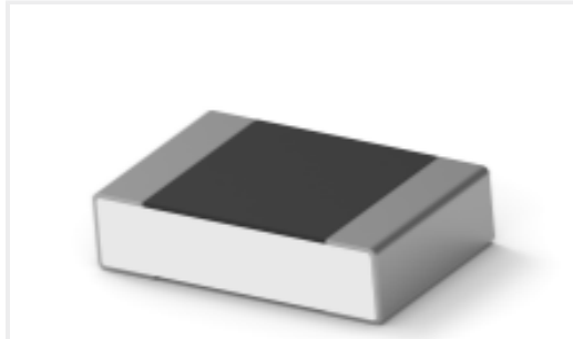
TE Part #8-2176379-2 RQ 0805 750R 0.1% 10PPM 5K RL
