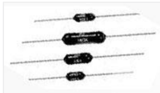
TE Part #7-1879625-1 H8 8K2 1% 50PPM
