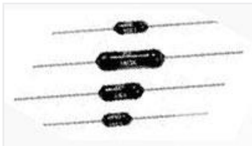
TE Part #3-1879625-2 H8 200R 1% 50PPM
