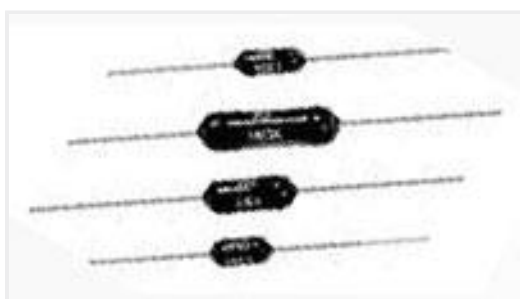
TE Part #9-1879639-7 H4P 1K0 0.5% 50PPM
