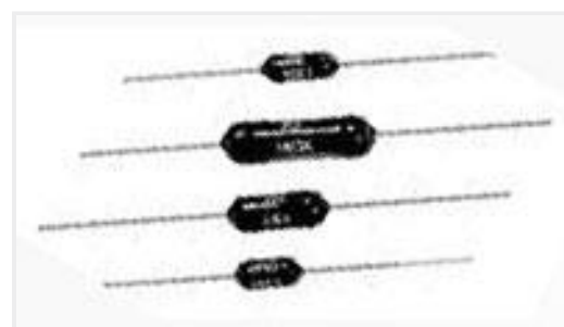
TE Part #3-1879629-1 H4P 47K 0.5% 100PPM
