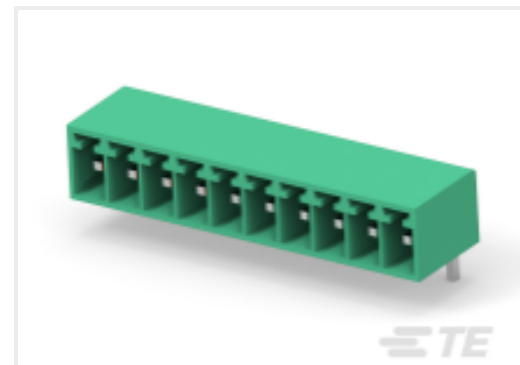
TE Part #1-2350514-0 10POS TB HDR 90 DEG, PITCH 3.5 &TL 3.5mm
