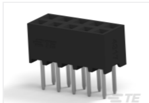
TE Part # 1-2307780-0 10P,2MM,B-B,REC,DRVT,2.7,0.1AU,TR, W/CAP
