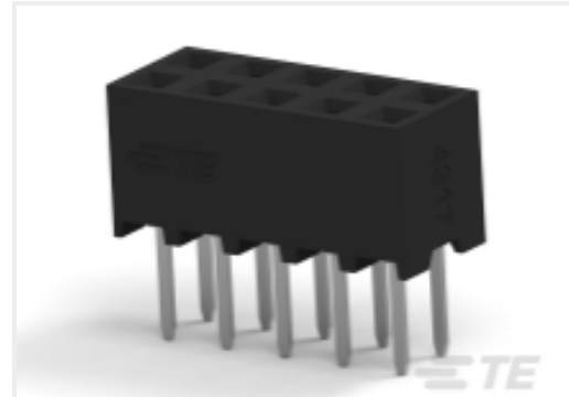
TE Part # 1-2307781-0 10P,2MM,B-B,REC,DRVT,3.2,0.1AU, TUBE
