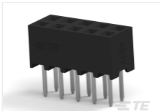
TE Part # 1-2314812-0 10P,2MM,B-B,REC,DRVT,2.0,0.1AU,TB, W/CAP
