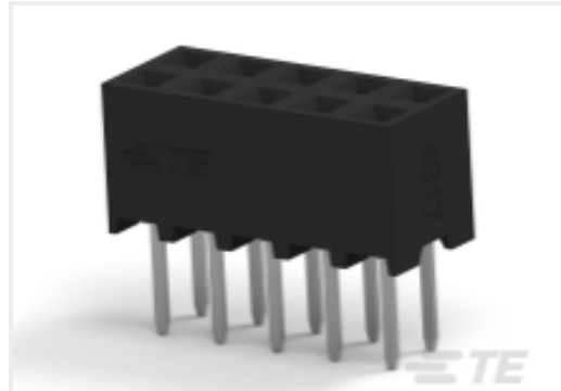
TE Part # 1-2314824-0 10P,2MM,B-B,REC,DRVT,2.7,0.1AU,TB, W/CAP
