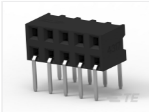
TE Part # 1-2307721-2 12P,2MM,B-B,REC,DRHZ,2.1,0.76AU,TR
