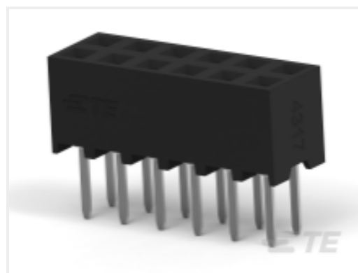
TE Part # 1-2307786-2 12P,2MM,B-B,REC,DRVT,2.7,0.76AU, TR,W/CAP
