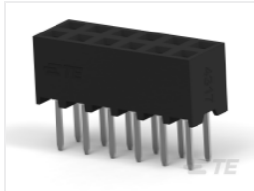
TE Part # 1-2307787-2 12P,2MM,B-B,REC,DRVT,3.2,0.76AU, TUBE
