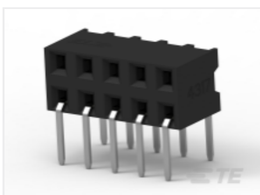
TE Part # 1-2307723-2 12P,2MM,B-B,REC,DRHZ,3.4,0.76AU, TUBE
