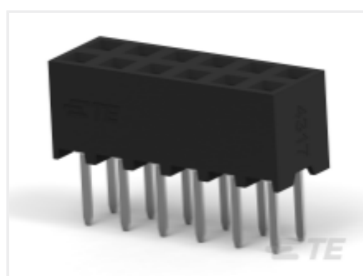
TE Part # 1-2314826-2 12P,2MM,B-B,REC,DRVT,2.7,0.76AU, TB,W/CAP
