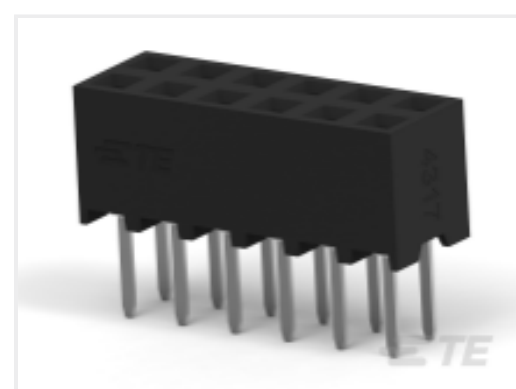
TE Part # 1-2314814-2 12P,2MM,B-B,REC,DRVT,2.0,0.76AU, TB,W/CAP
