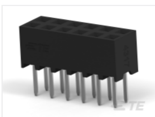
TE Part # 1-2307785-2 12P,2MM,B-B,REC,DRVT,2.0,0.76AU, TR,W/CAP
