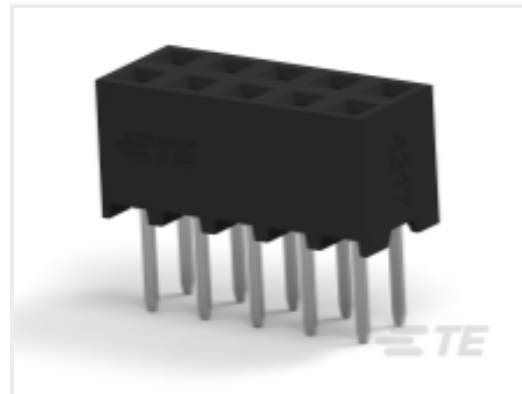
TE Part # 1-2307785-0 10P,2MM,B-B,REC,DRV,2.0,0.76AU, TR,W/CAP
