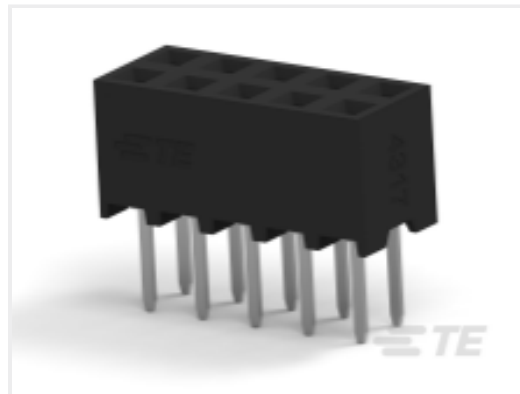
TE Part # 1-2307787-0 10P,2MM,B-B,REC,DRV,3.2,0.76AU, TUBE
