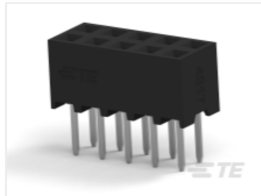
TE Part # 1-2307786-0 10P,2MM,B-B,REC,DRV,2.7,0.76AU, TR,W/CAP
