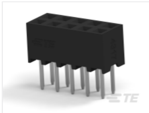
TE Part # 1-2314822-0 10P,2MM,B-B,REC,DRV,2.7,0.76AU,TB
