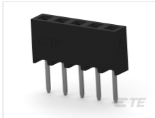
TE Part # 2307773-5 5P,2MM,BB,REC,SRVT,2.0,0.76AU,TR, W/CP
