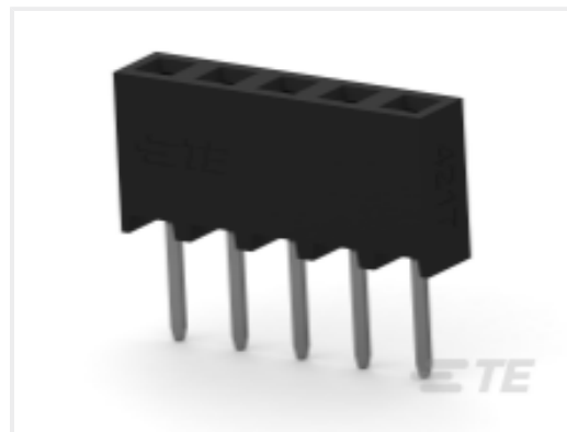
TE Part # 2307775-5 5P,2MM,B-B,REC,SRVT,3.2,0.76AU, TUBE
