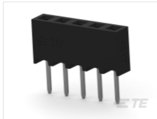
TE Part # 2314882-5 5P,2MM,BB,REC,SRVT,2.7,0.76AU,TB, W/CP
