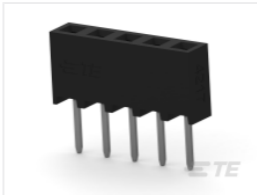
TE Part # 2307774-5 5P,2MM,BB,REC,SRVT,2.7,0.76AU,TR, W/CP
