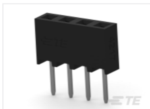
TE Part # 2314876-4 4P,2MM,B-B,REC,SRVT,2.7,0.1AU,TB
