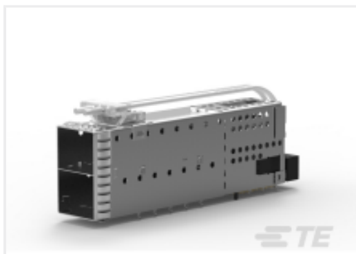
TE Part # 2-2296273-1 MICROQSFP 2X1 CAGE ASSY EMI SPRING, 2LP
