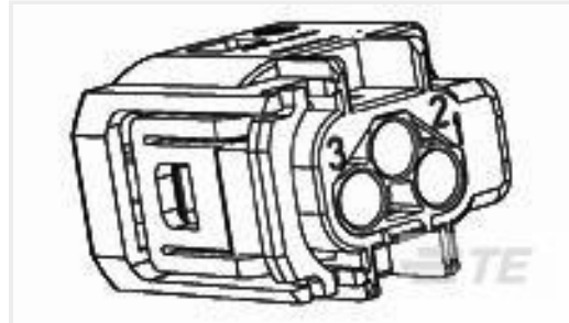
TE Part #1-967642-1 3POS MOS REC SEALED COD A
