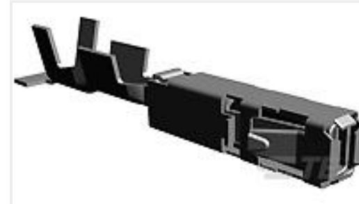
TE Part #1-1241380-2 AMP MCP 1.5K, CONTACT, SWS
