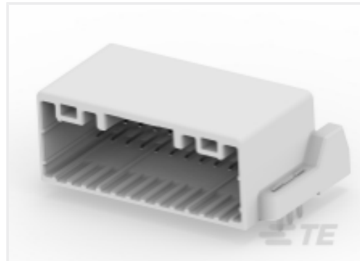
TE Part #2237067-4 24POS,TAB0.64X0.64,HDR ASSY,90 DEG,SMD
