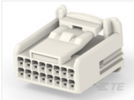
TE Part # 1717109-1 0.64 III 16POS PLUG ASSY
