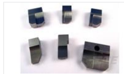
TE Part #3-1633107-9 ANVIL, COMBINATION
