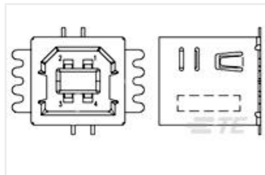
TE Part #1734517-1 STD USB TYPE B, VERTICAL, SMT, GRD FINGER
