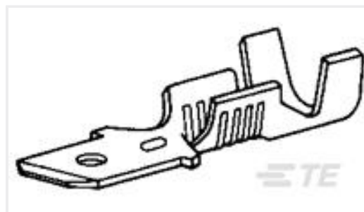
TE Part #62531-1 205 FASTON TAB 18-14 AWG TPBR
