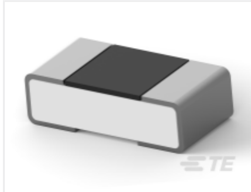
TE Part #4-2176363-4 RQ 0402 1K21 0.1% 10PPM 5K RL
