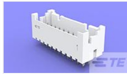
TE Part #3-1969570-0 ASSY,HDR,VERT,GWT,BOSS,DUAL ROW, EP2.5
