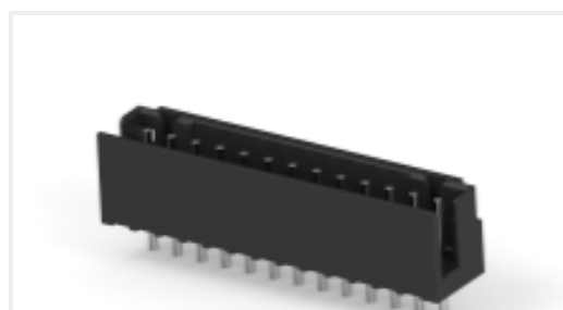
TE Part # CAT-3980407-RHDRRA CT 2mm Header Assembly: Right Angle
