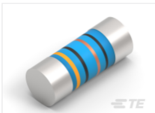
TE Part #2176314-1 MELF SMA_A 100R 0.1% 15PPM 0102 0.3W
