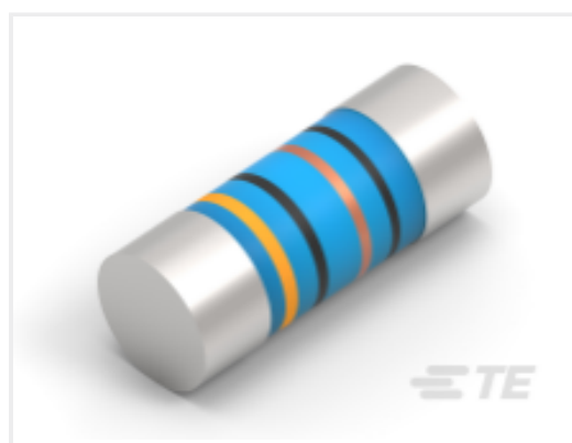
TE Part #2176335-7 MELF SMA-A 36R 1% 50PPM 0102 0.3 W
