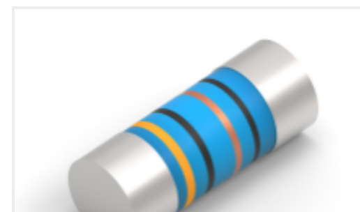
TE Part #2176334-9 MELF SMA-A R43 1% 50PPM 0204 0.4 W
