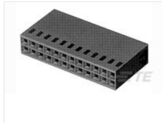
TE Part #87456-7 12 MODIV HSG COMP DR .100CL
