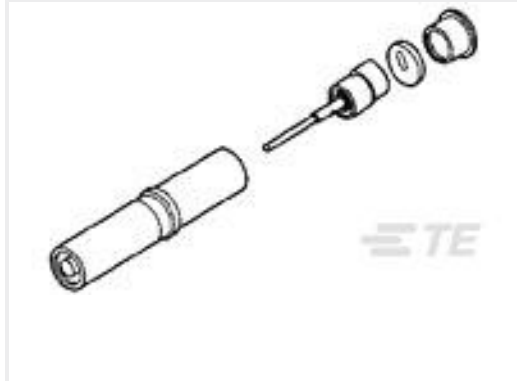
TE Part #1218820-1 COAX SZ 8 ARINC SOCKET CONTACT
