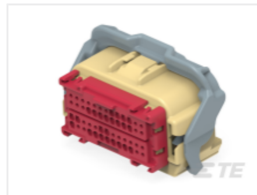
TE Part #1-2296315-3 ACU 52P PLUG ASSY(B2B4)
