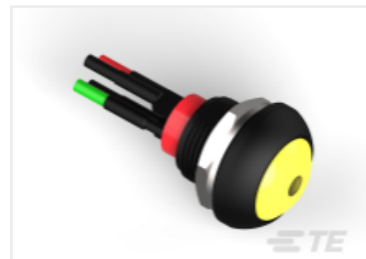
TE Part #1-2329389-1 PB OFF/ON FC YLW M1 TERM WHI LED IP68 50
