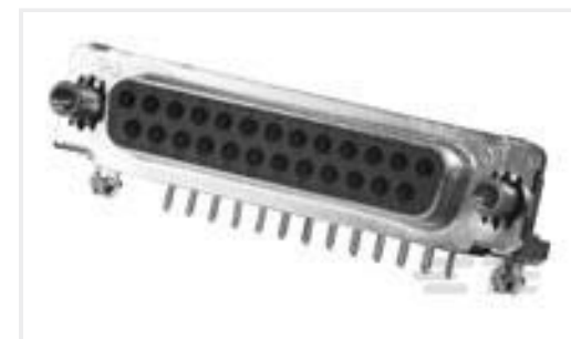
TE Part #5745782-2 15 MSFL RCPT RA 318 (FM)
