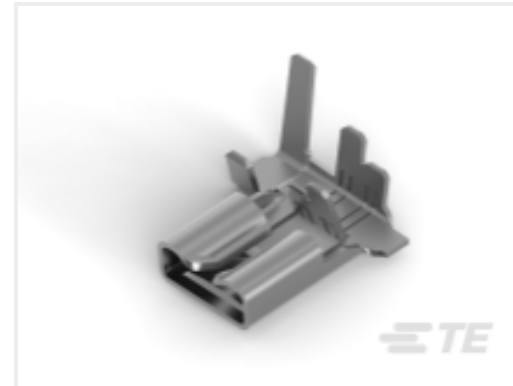
TE Part # 2238171-3 250 FASTON, FLAG, REC., 22-12 AWG, TPBR
